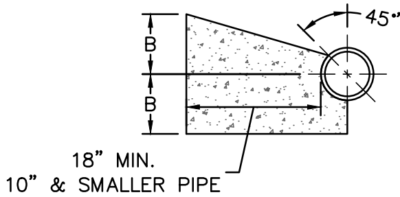
SECTION X-X BENDS & TEES
