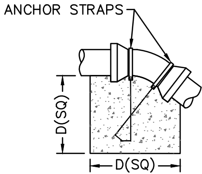
45° VERTICAL BENDS
