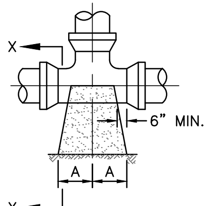
PLAN TEES
