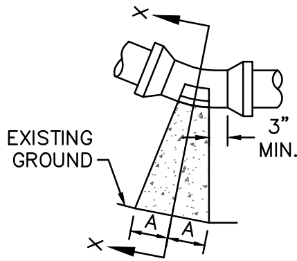
PLAN BENDS
