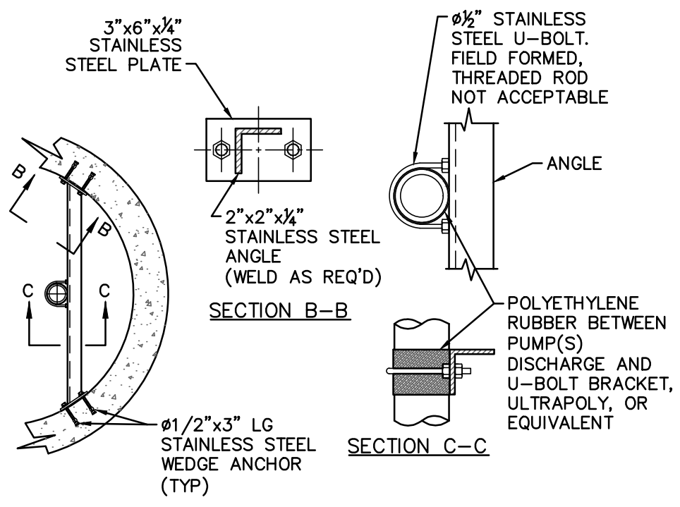
BRACKET DETAILS AND SECTIONS NOT TO SCALE
